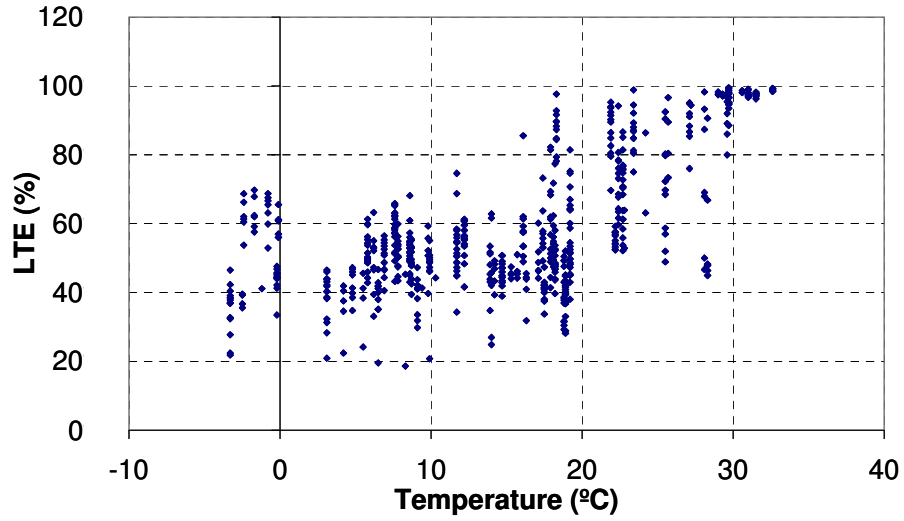
Figure 117. Computed LTE versus PCC temperature for nondoweled section 31–3018.
