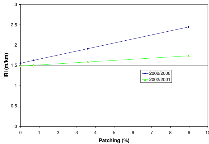
Figure 58. Effect of percent patching on IRI for the 1–37A models.
