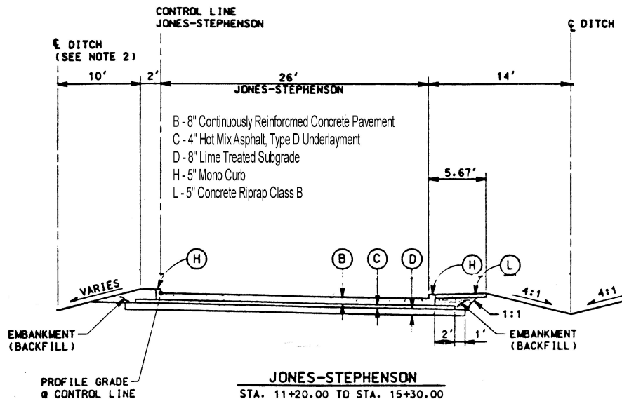
Figure 86. Typical cross section for the CRCP instrumented section.
