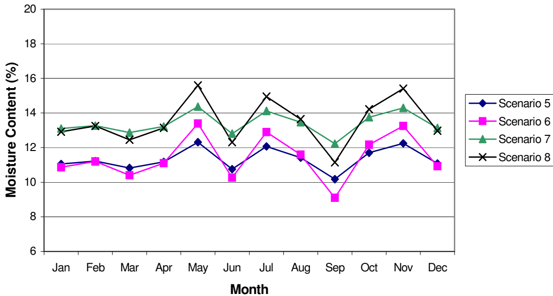
Figure 23. Monthly moisture content variation for well-graded silty gravel (GW-GM), scenarios 5–8.
