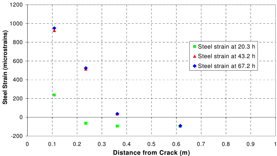
Figure 182. Steel strain along the slab length at different ages.
