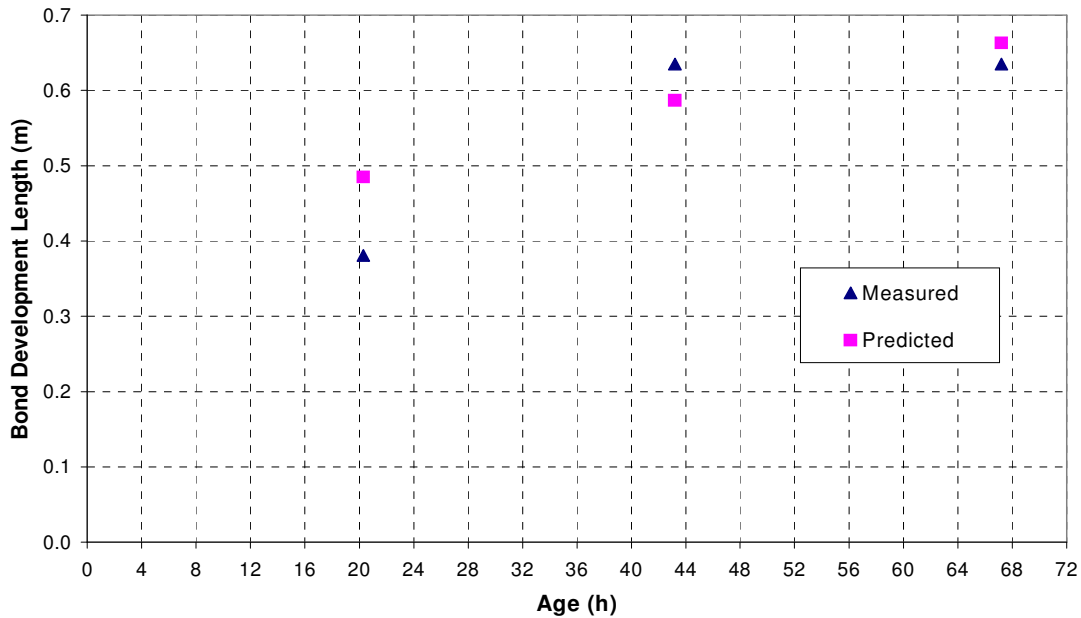
Figure 186. Comparison of measured and predicted bond development length.
