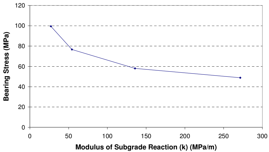
Figure 72. Effect of varying the modulus of subgrade reaction (k) on the bearing stress.
