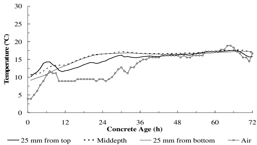
Figure 236. Measured concrete and air temperatures for Minnesota, Slab 3.
