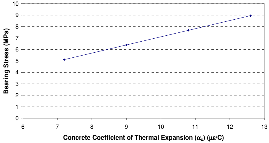
Figure 69. Effect of varying the concrete CTE ( \alpha_c ) on the bearing stress.
