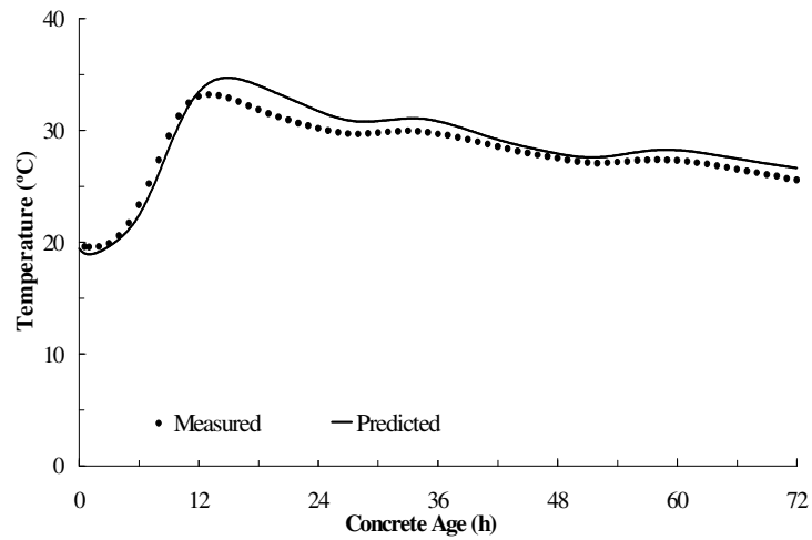
Figure 218. Measured versus predicted temperatures 25 mm from bottom of slab for Lufkin, TX, Slab 2.
