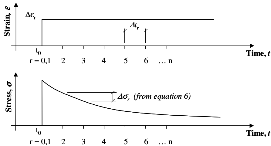
Figure 17. Discretized subdivision of time for numerical creep analysis.
