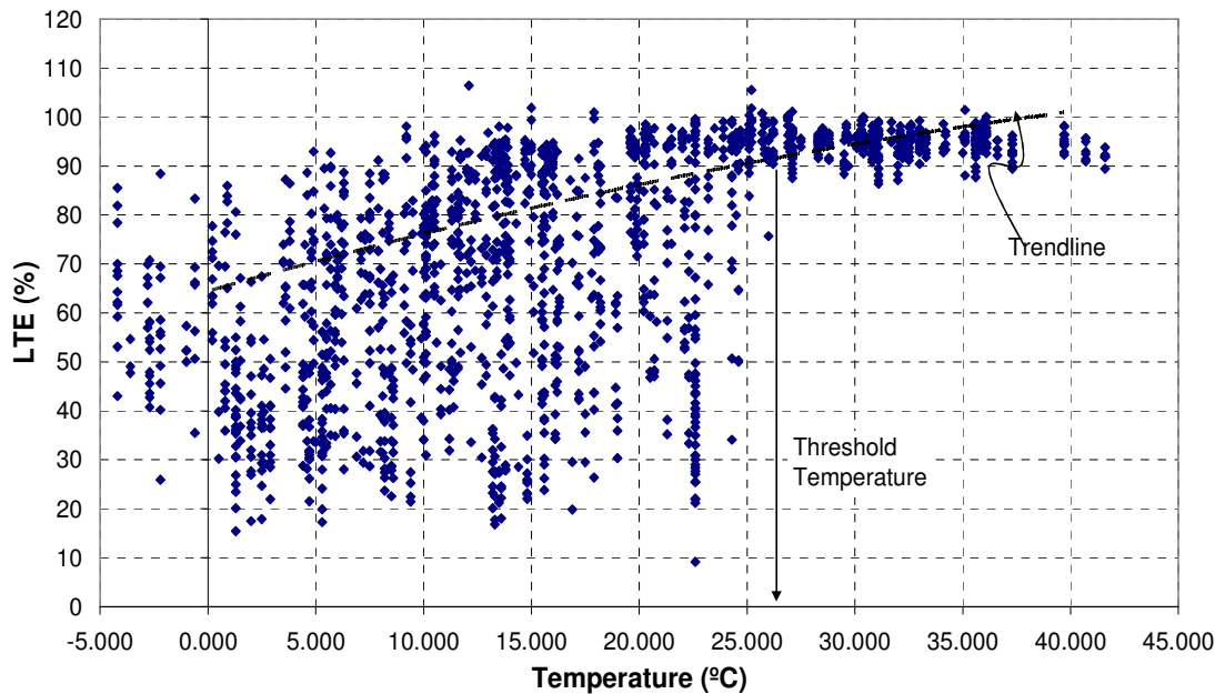
Figure 113. Computed LTE versus PCC temperature for section 49–3011.
