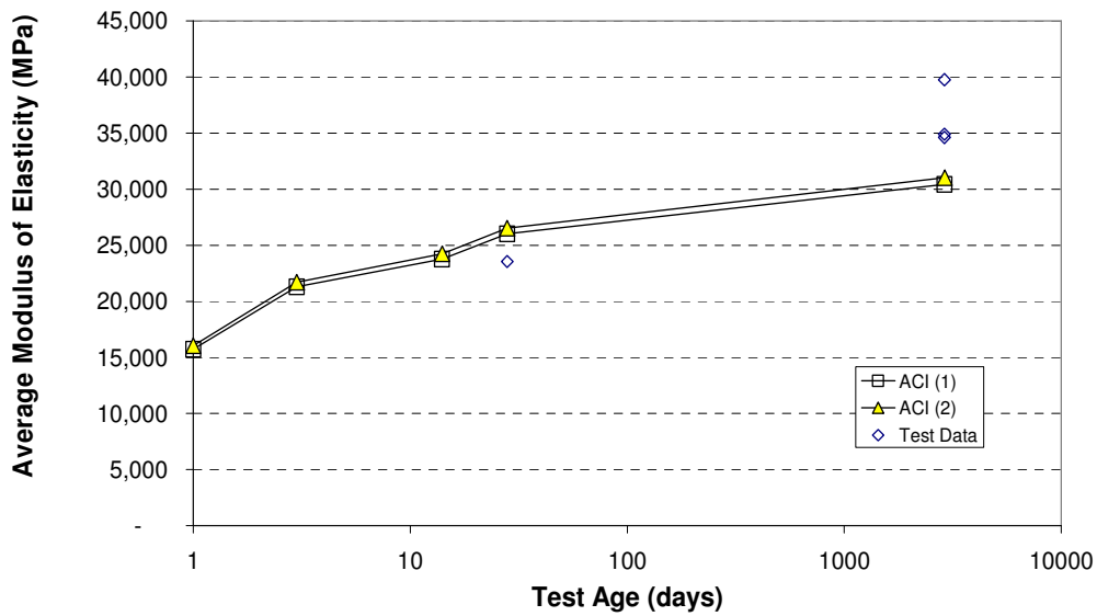
Figure 103. Time growth of Mexico modulus of elasticity.
