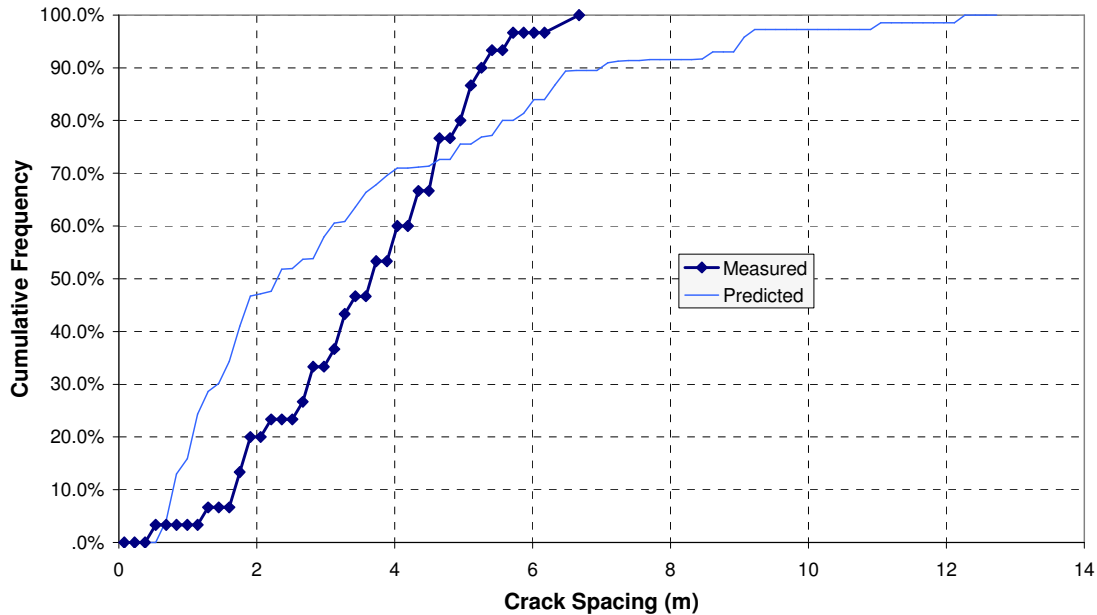
Figure 178. Measured versus predicted crack spacing at 3 days of age, Fort Worth, TX
