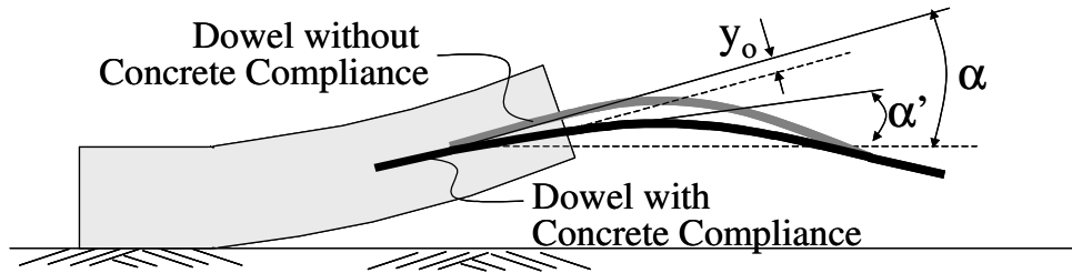
Figure 64. Schematic of dowel deformation without concrete compliance and with concrete compliance at the joint.
