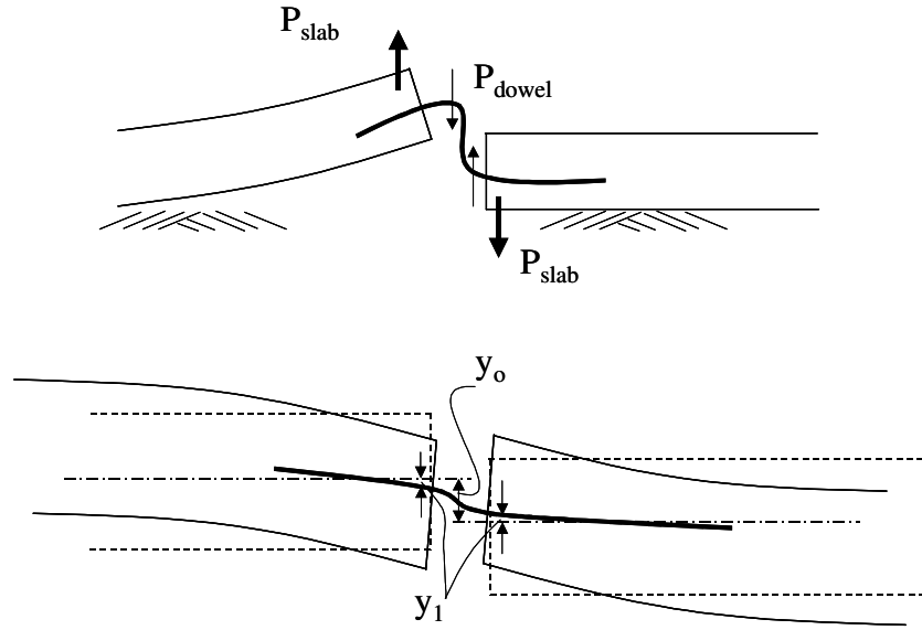
Figure 74. Schematic representation of slabs loaded in shear.
