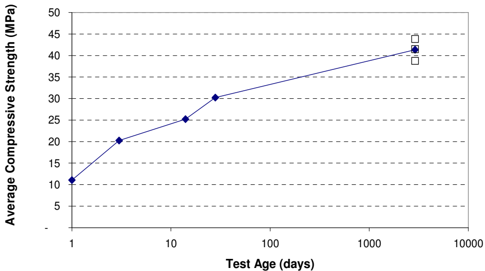
Figure 101. Time growth of Mexico compressive strength.
