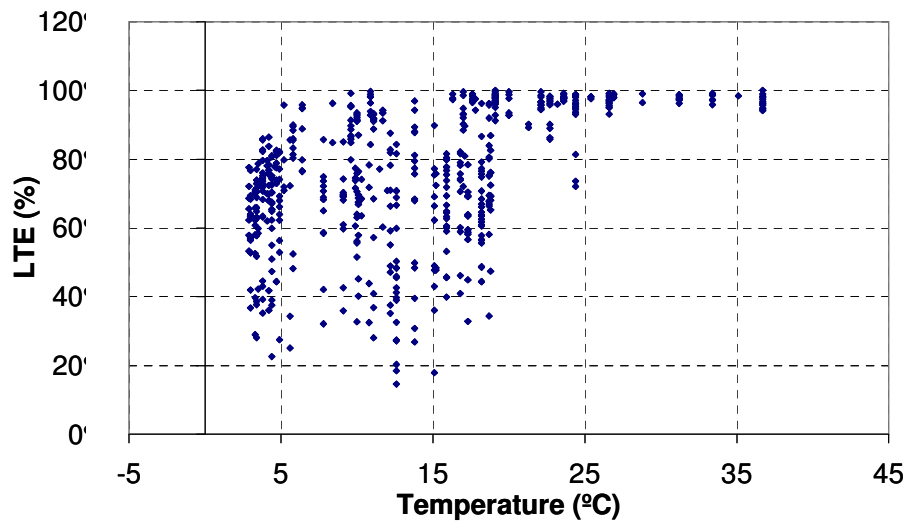
Figure 118. Computed LTE versus PCC temperature for nondoweled section 06–3042.
