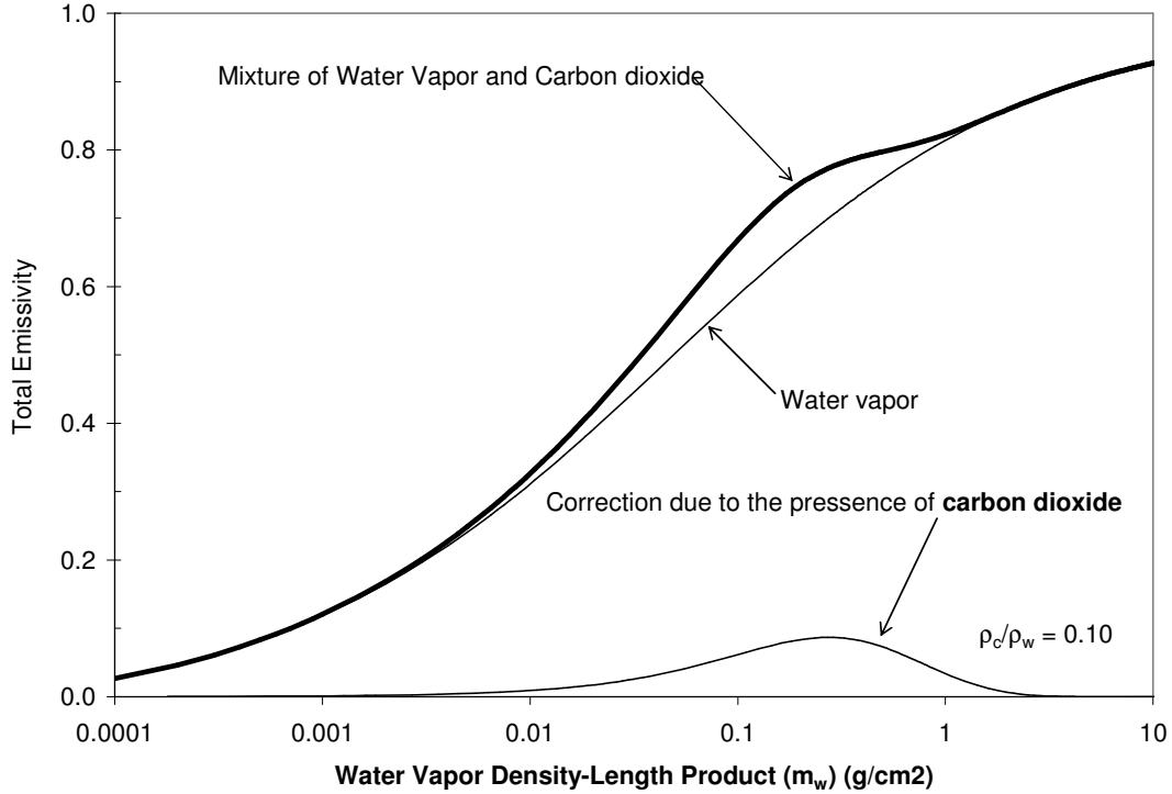
Figure 6. Emissivity of moist air at a total pressure of 1 atmosphere and a temperature of 20 °C.
