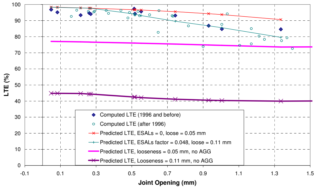
Figure 135. Predicted versus computed LTE for section 37–0201, joint 145.1 m from start of section.
