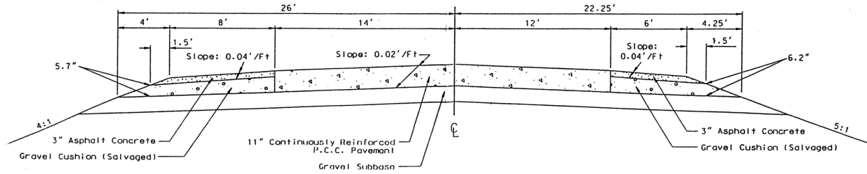
Figure 91. Typical cross section for I-29, South Dakota (from opposite direction to traffic).
