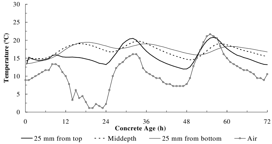
Figure 196. Measured concrete and air temperatures for Minnesota, Slab 1.
